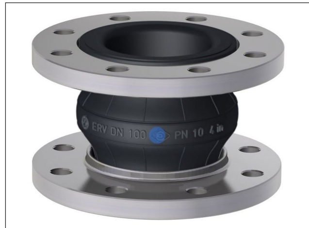
ERV-BR, special type for abrasive media. Available in DN 25 to 300 mm.
